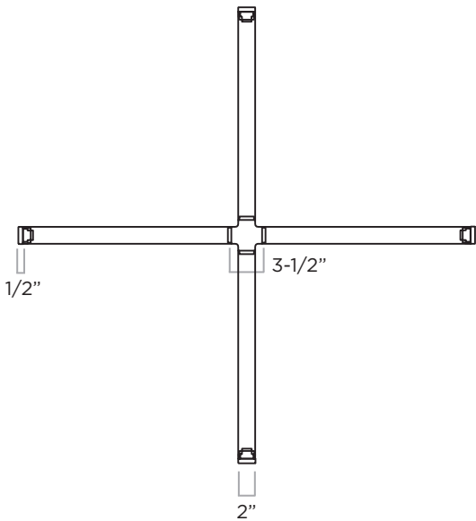
4-WAY
